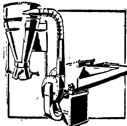
WARDS ALL STEEL M-15 HAMMERMILL 135.00 See it! It's a better, big capacity mill for less money! Swinging hammers!
